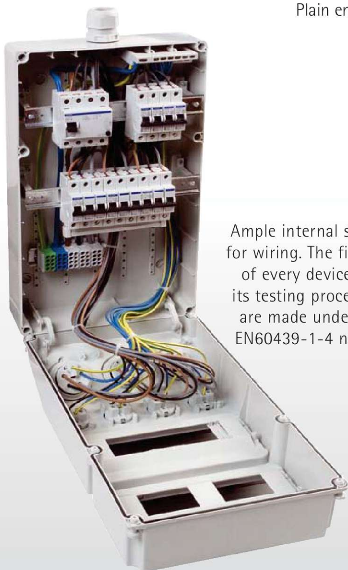
Plain enclosure
